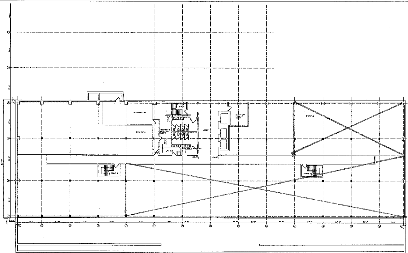
EXISTING LOWER FLOOR PLAN SCALE 1/8" = 1'-0"
