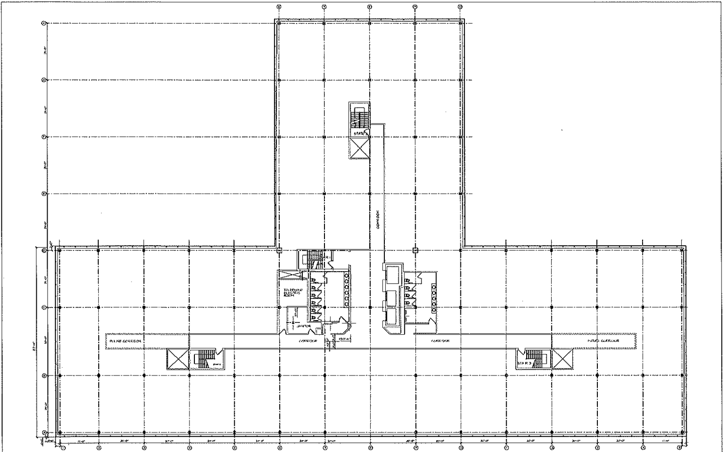
PROPOSED THIRD AND FOURTH FLOOR PLAN SCALE: 1/8" = 1'-0"
