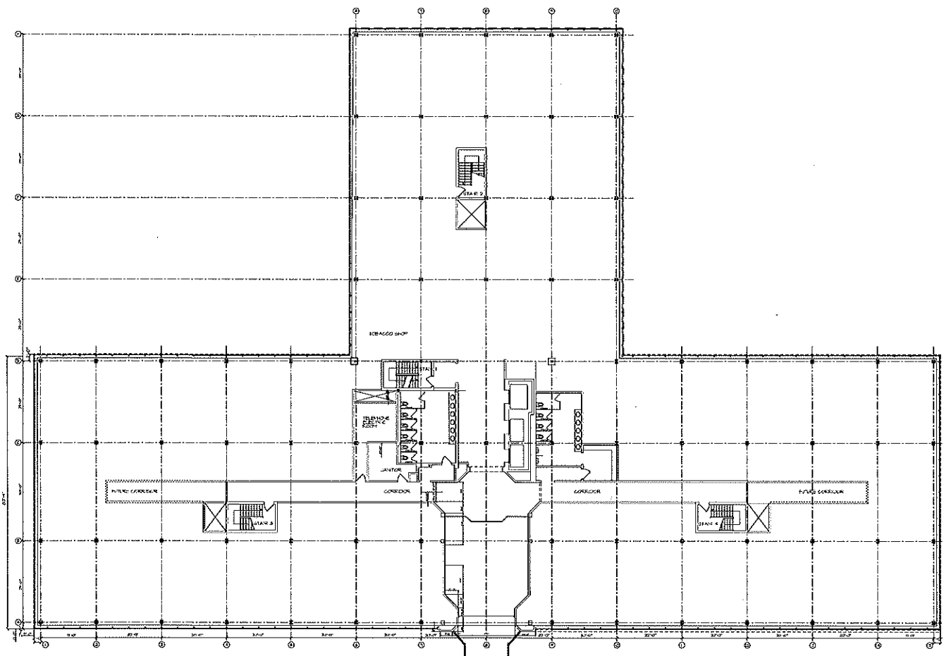
PROPOSED SECOND FLOOR FRAMING PLAN SCALE 1/8" = 1'-0"
